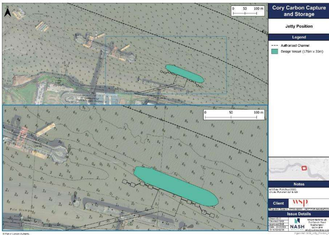
Figure 4: Jetty Option B
