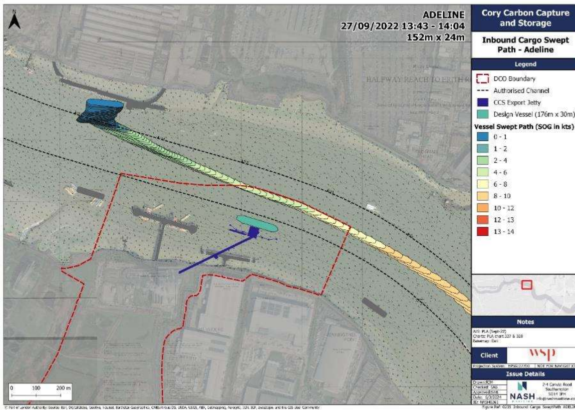
Figure 30: Swept Path Ford's Jetty Arrival ( Adeline )
